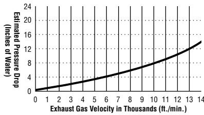
Pressure Drop, Standard Units
