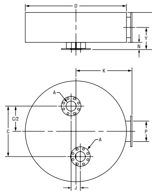
Dual Inlet Type 2
