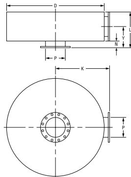
Single Inlet
