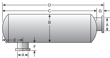
Side-In, End-Out Design
