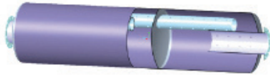
Multi-chamber exhaust silencers for most reciprocating engines.
