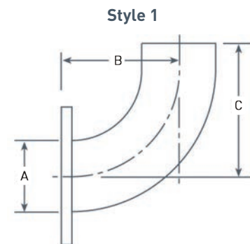
ANSI Light Flange Connection
