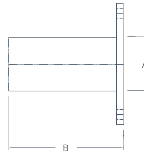
Sizes 4-12" – ANSI Light Flange Connection Sizes 14-22" – 125/150# ANSI Flange Connection
