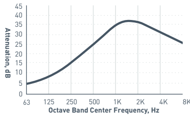
Typical Attenuation Curve SU4 Series
