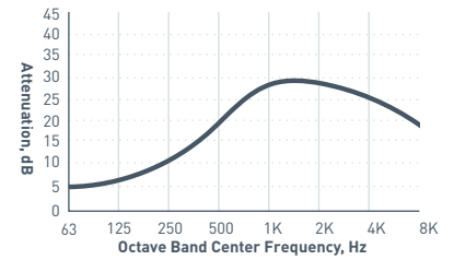
Typical Attenuation Curve SU3 Series
