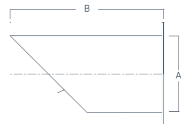
Sizes 4-12" – ANSI Light Flange Connection Sizes 14-22" – 125/150# ANSI Flange Connection
