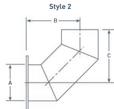
Sizes 8"–12" - ANSI Light Flange Connection Sizes 14"–22" - 125/150# ANSI Flange Connection
