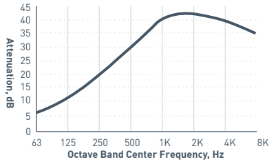
Typical Attenuation Curve SU5 Series
