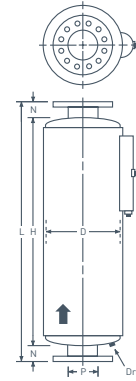
End-In, End-Out Design
