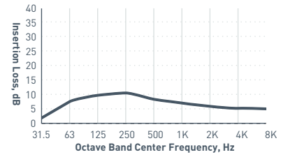
Typical Insertion Loss
